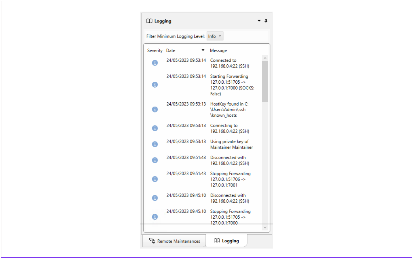
Figure 3.8: Logging
