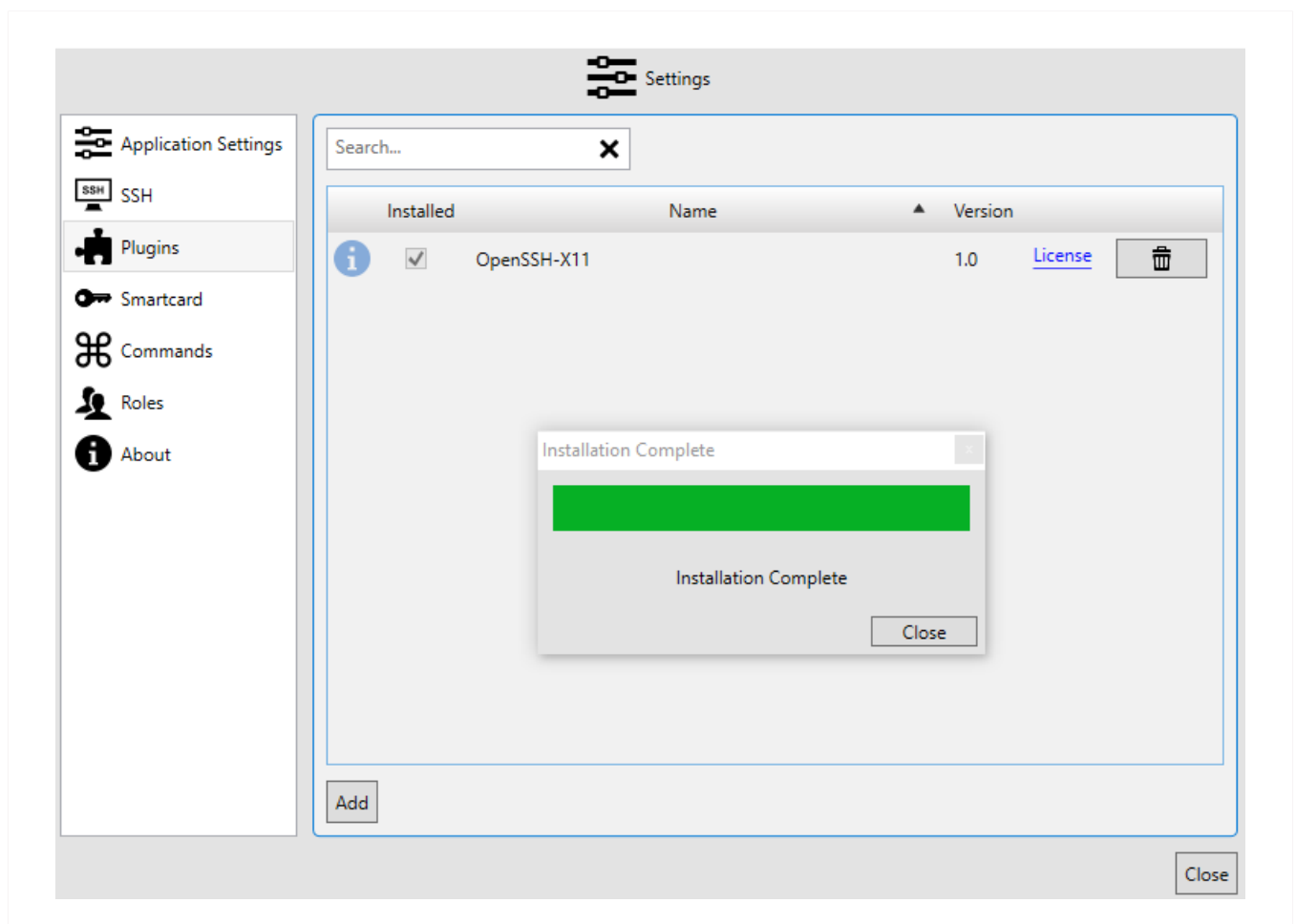
Figure 3.13: Plugins
