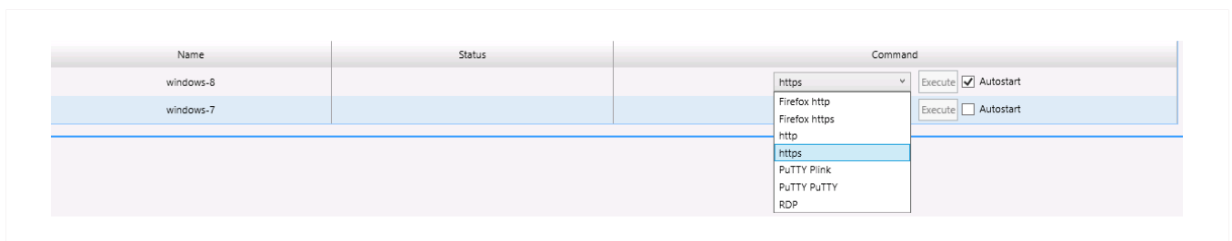
Figure 3.12: Autostart Function
