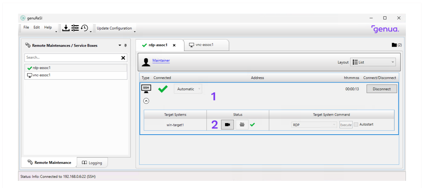
Figure 3.2: Window Layout
