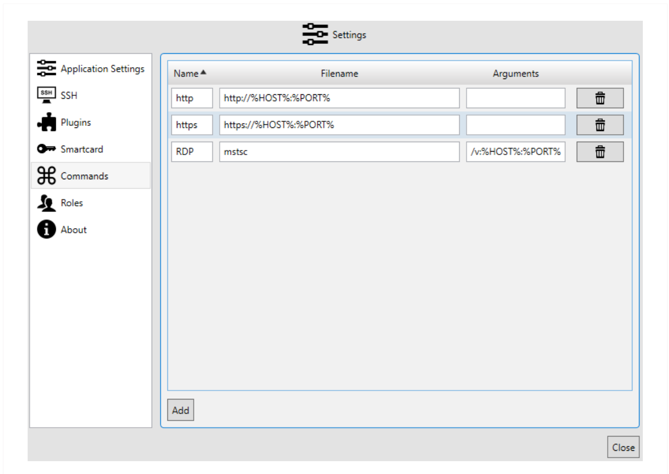
Figure 3.11: Commands Settings
