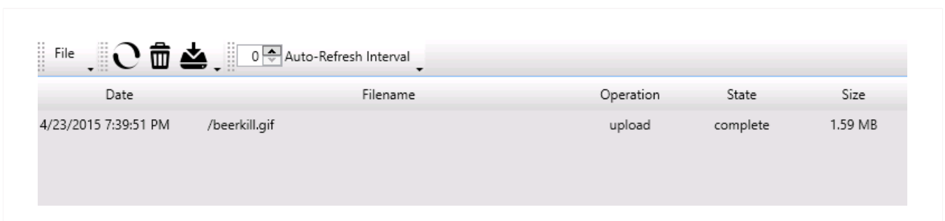
Figure 4.7: File Exchange
