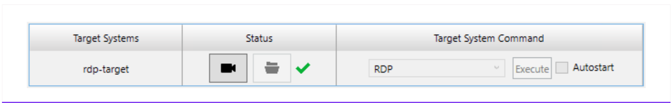
Figure 3.4: Recording Connections
