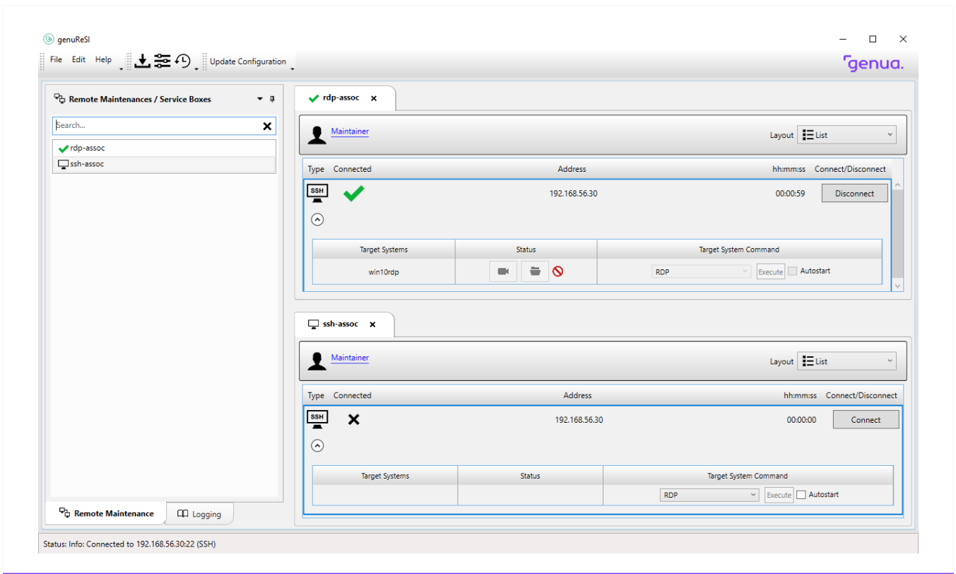
Figure 5.5: GUI Layout
